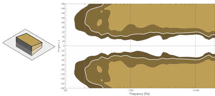
Loudspeaker directivity (using the 110° setting) in horizontal plane using lines of equal sound pressure at -3 dB, -6 dB, -12 dB.
